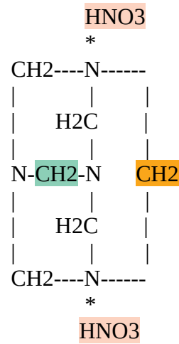
Hexamindinitrat
