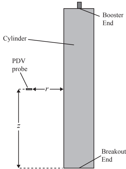
Figure 1. Experimental configuration for the 50.8 mm and 76.2 mm cylinder tests.
