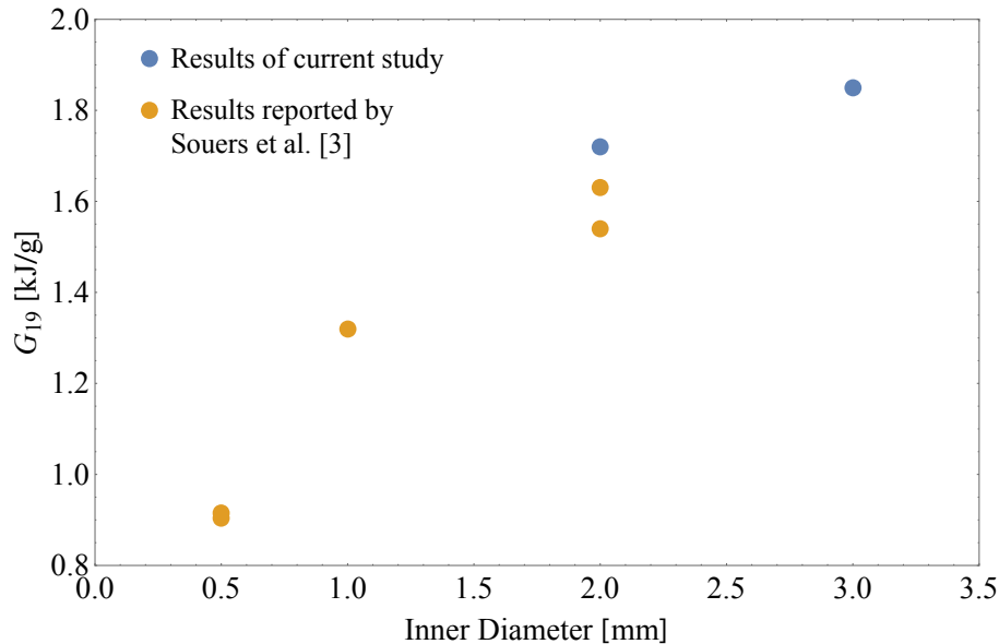
Figure 2. Gurney Energy computed at 19 mm scaled cylinder displacement for ammonal tests at various sizes.
